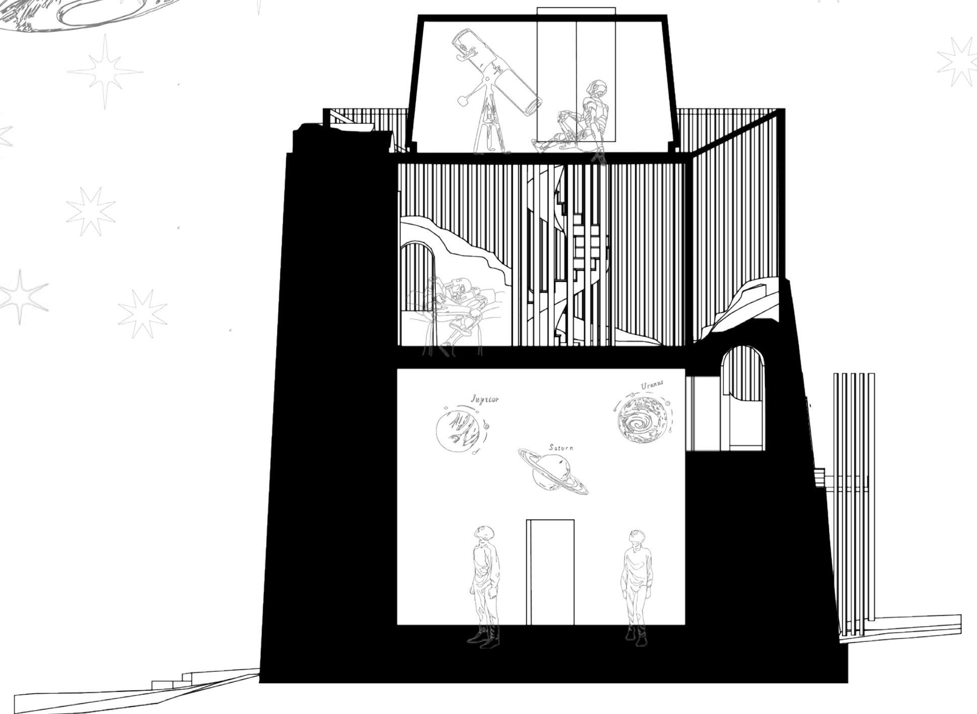
section 1:100
